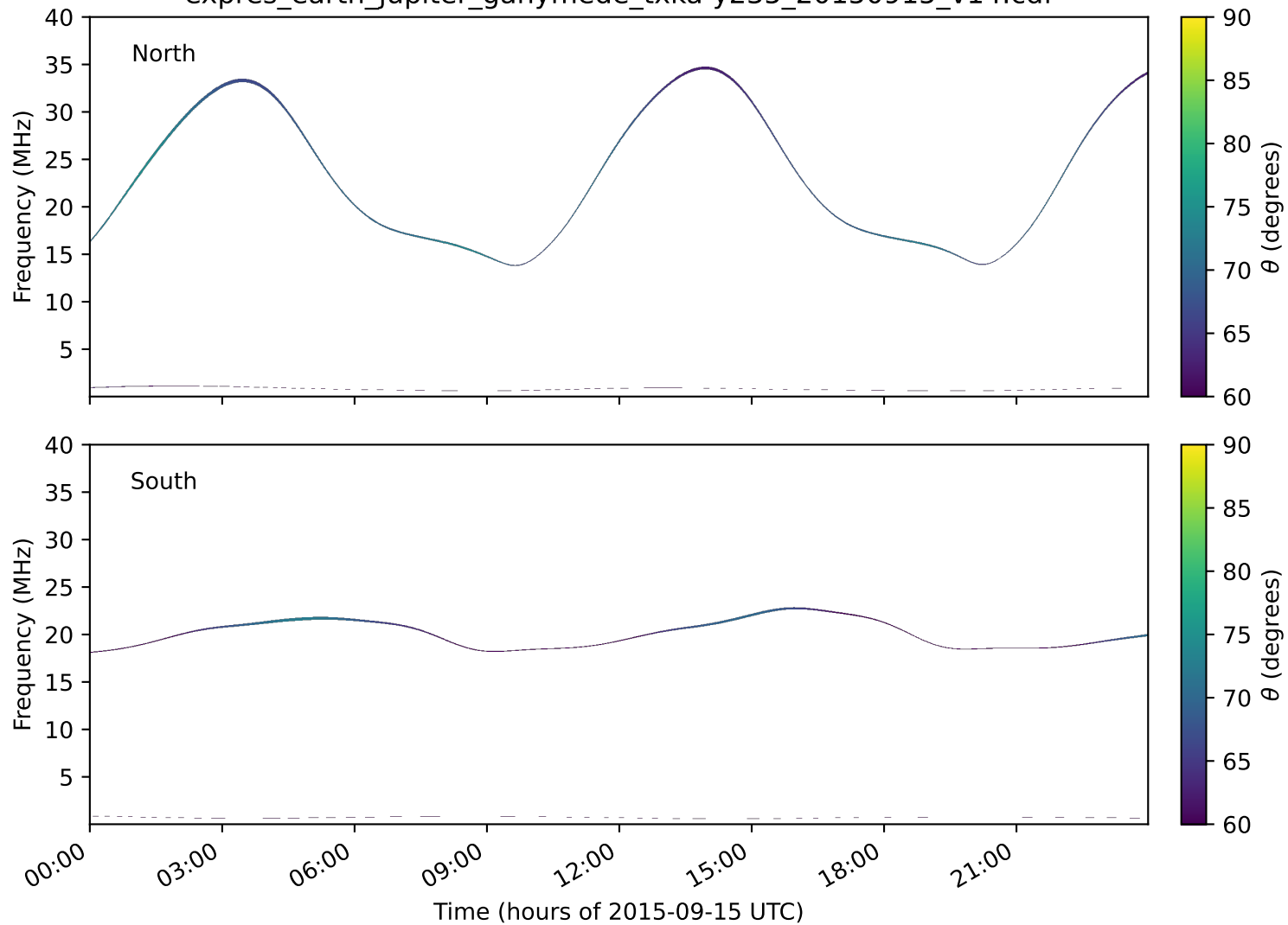
expres_earth_jupiter_ganymede_txka-y235_20150915_v14.cdf
