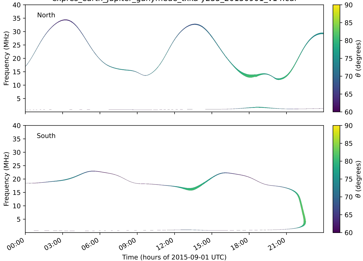
expres_earth_jupiter_ganymede_txka-y235_20150901_v14.cdf
