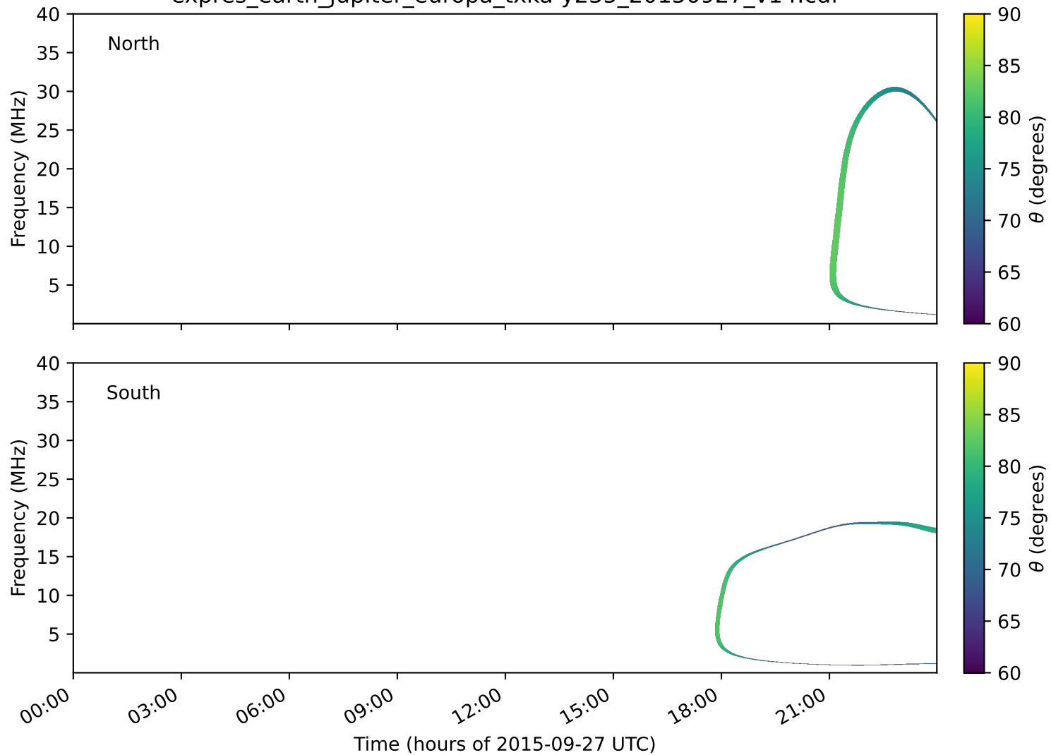
expres_earth_jupiter_europa_txka-y235_20150927_v14.cdf
