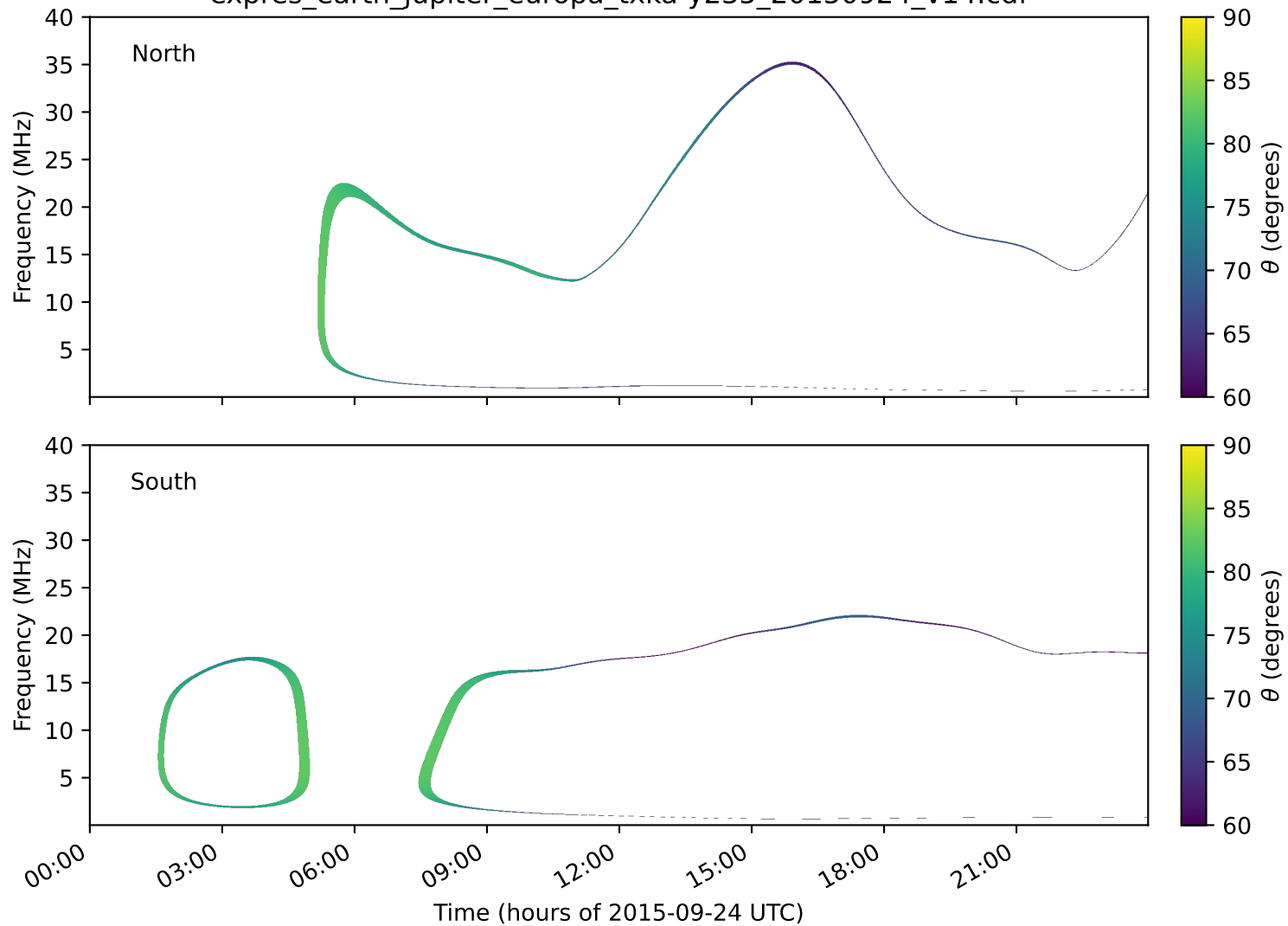
expres_earth_jupiter_europa_txka-y235_20150924_v14.cdf
