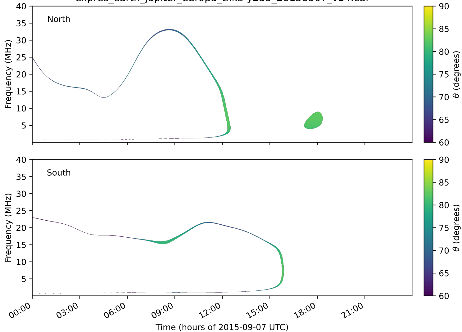
expres_earth_jupiter_europa_txka-y235_20150907_v14.cdf
