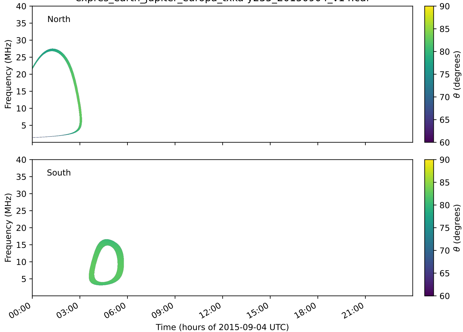
expres_earth_jupiter_europa_txka-y235_20150904_v14.cdf
