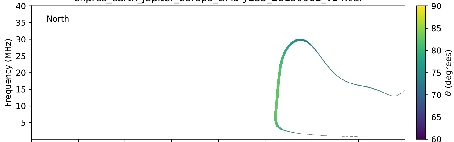
expres_earth_jupiter_europa_txka-y235_20150902_v14.cdf
