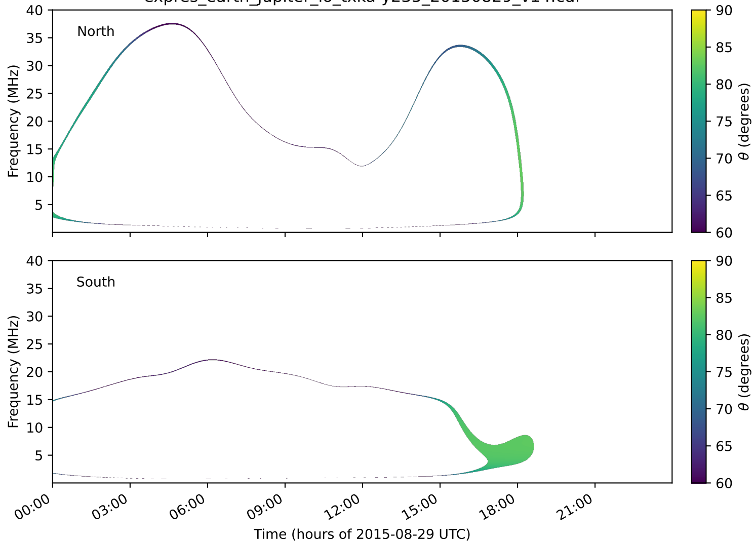
expres_earth_jupiter_io_txka-y235_20150829_v14.cdf
