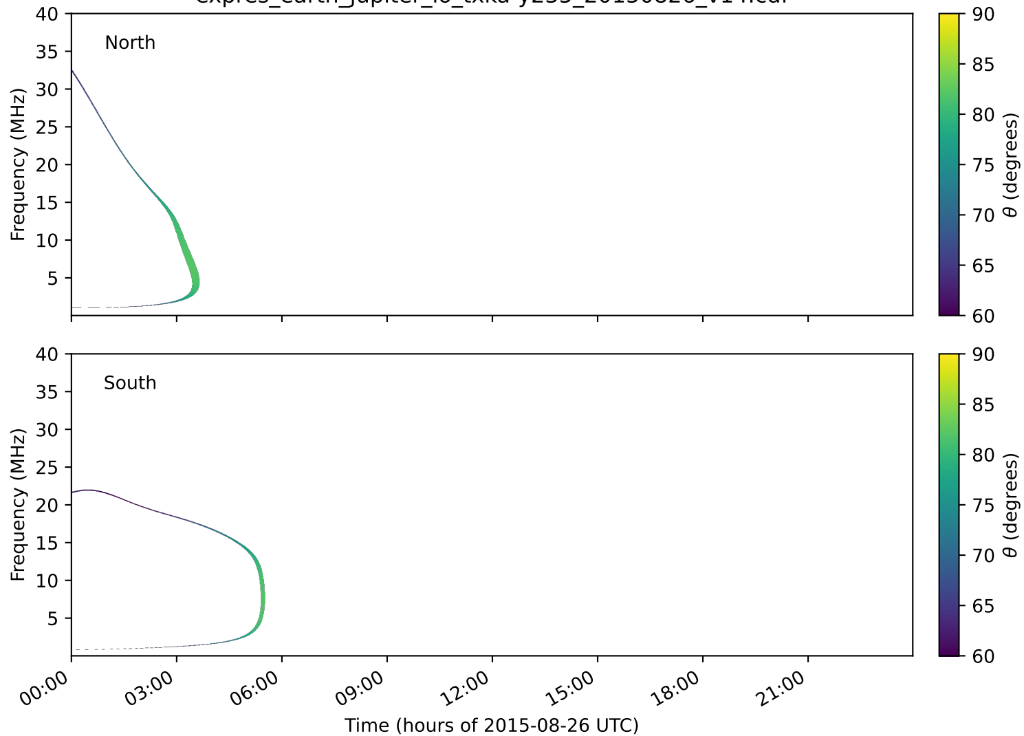
expres_earth_jupiter_io_txka-y235_20150826_v14.cdf
