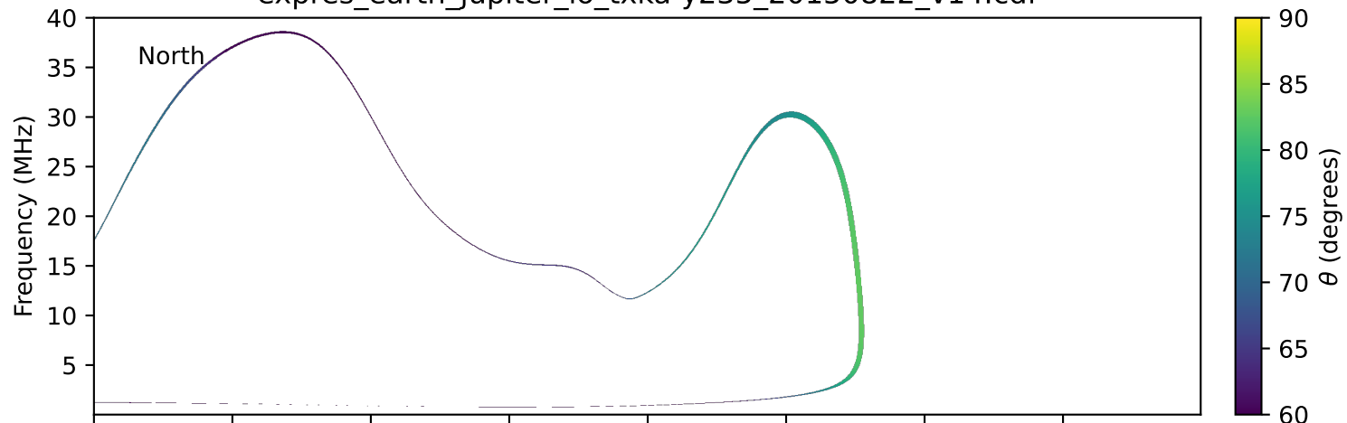
expres_earth_jupiter_io_txka-y235_20150822_v14.cdf
