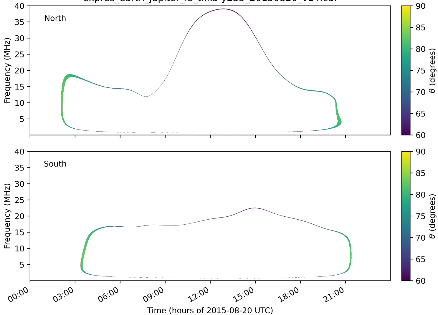
expres_earth_jupiter_io_txka-y235_20150820_v14.cdf
