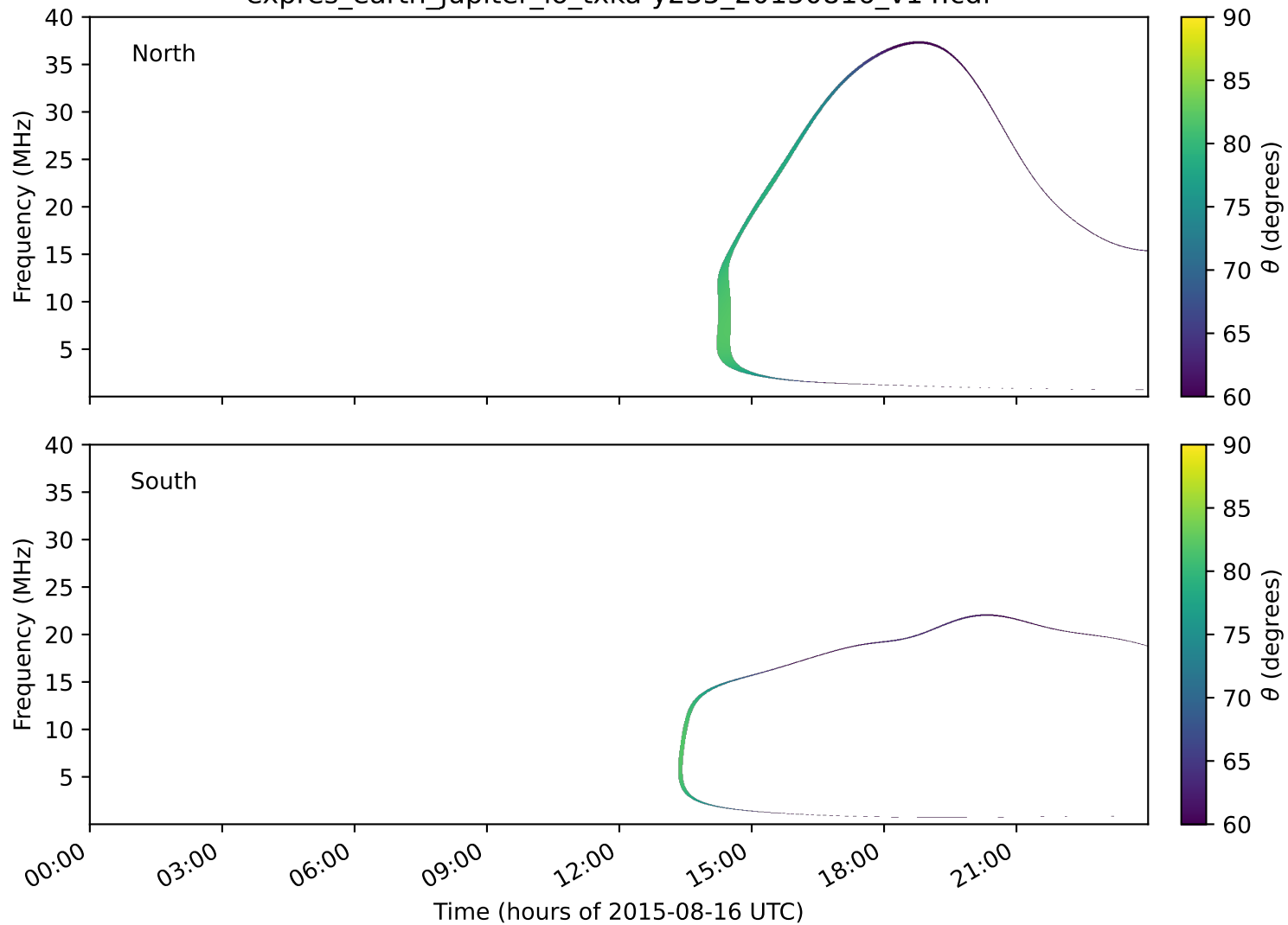
expres_earth_jupiter_io_txka-y235_20150816_v14.cdf
