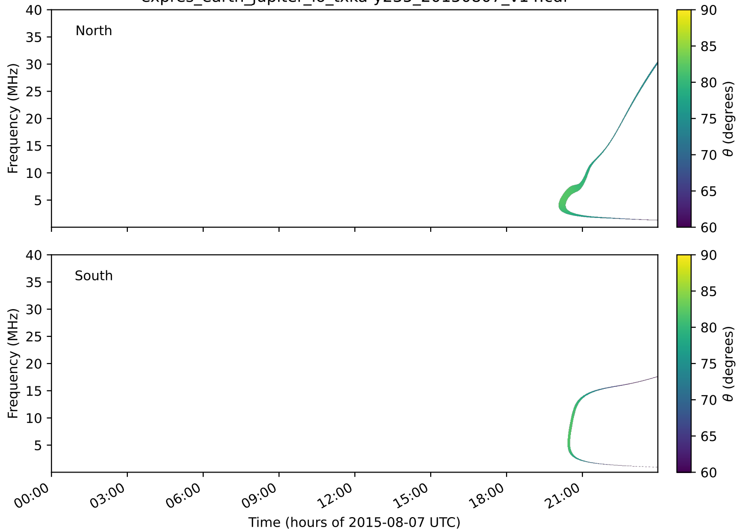
expres_earth_jupiter_io_txka-y235_20150807_v14.cdf
