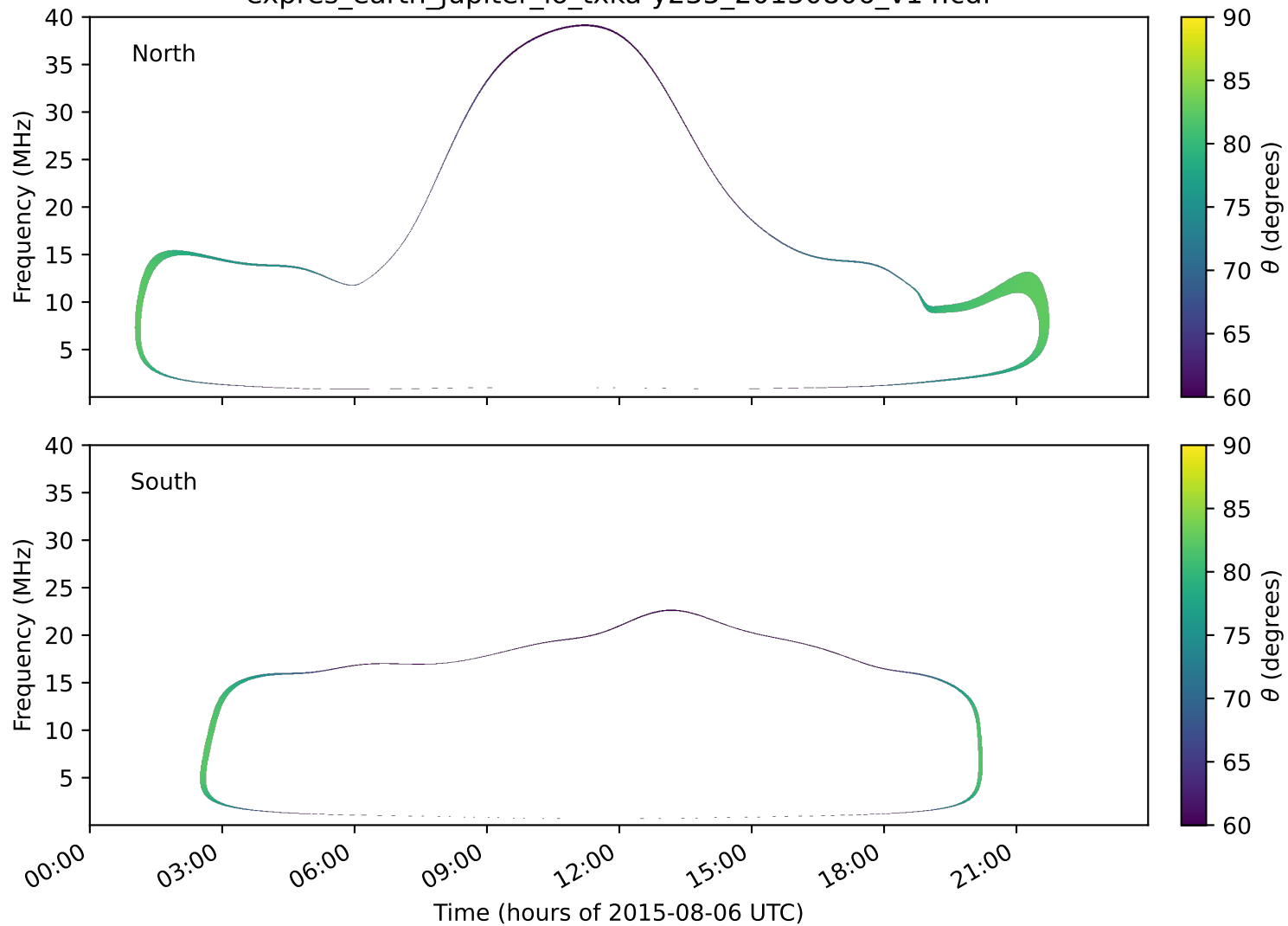
expres_earth_jupiter_io_txka-y235_20150806_v14.cdf
