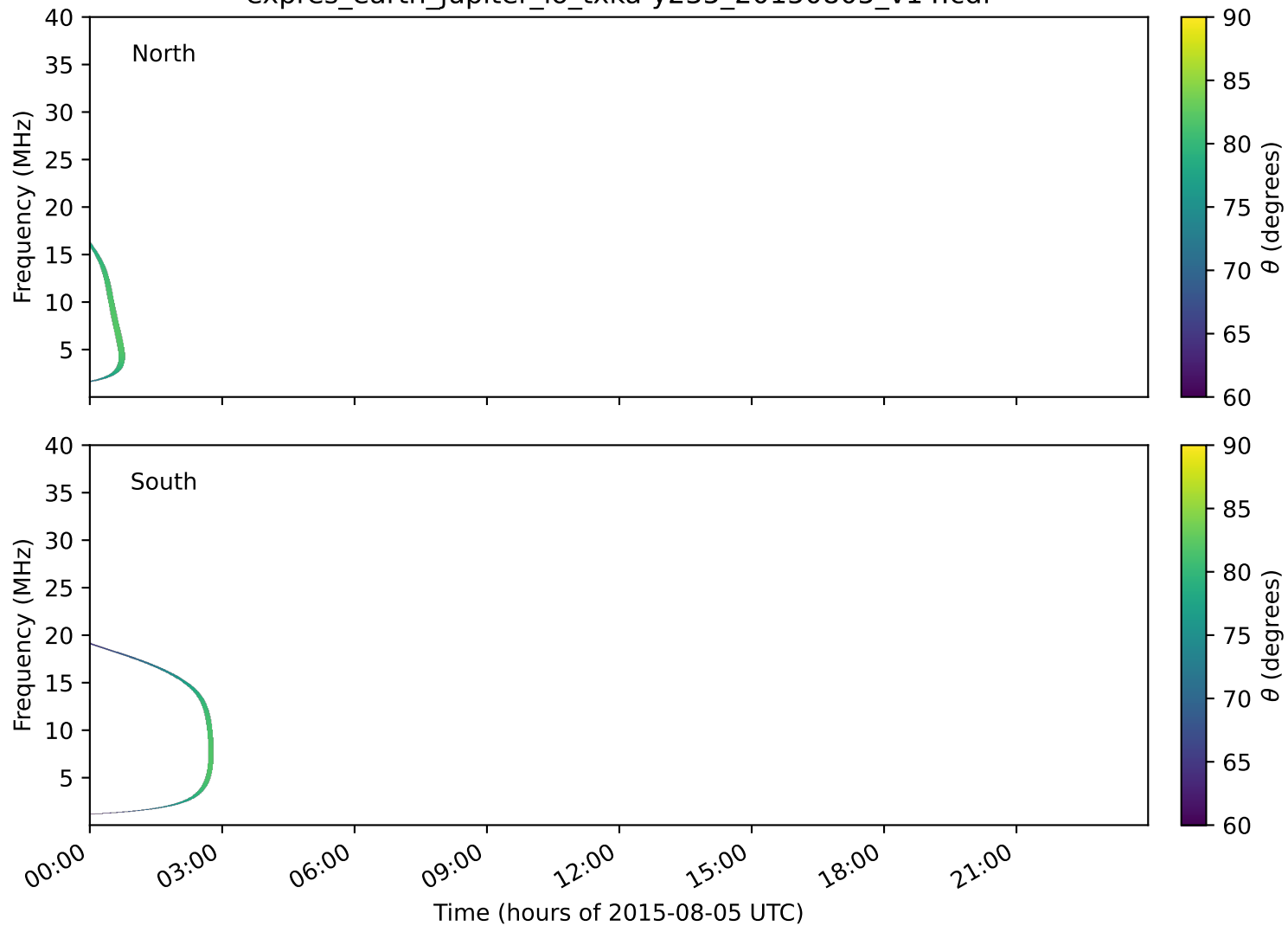
expres_earth_jupiter_io_txka-y235_20150805_v14.cdf
