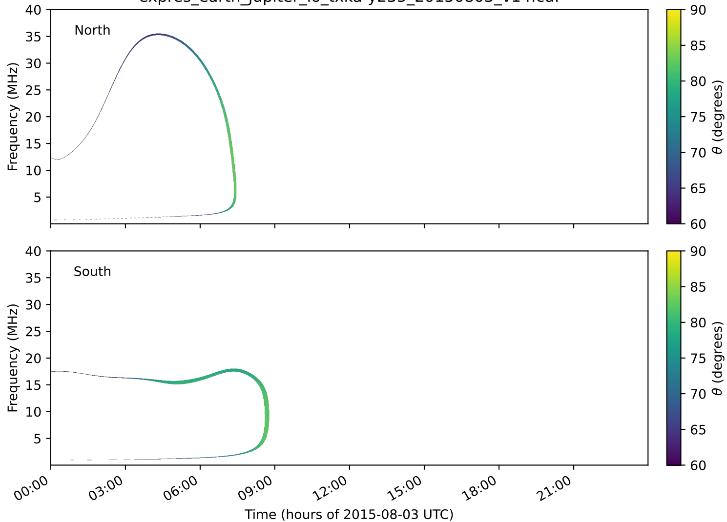
expres_earth_jupiter_io_txka-y235_20150803_v14.cdf
