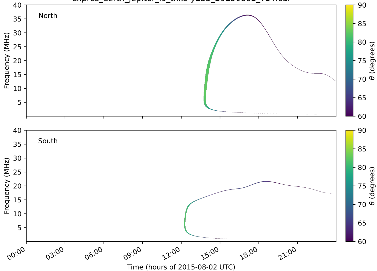
expres_earth_jupiter_io_txka-y235_20150802_v14.cdf
