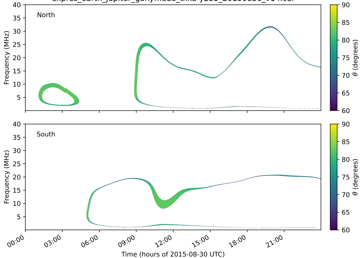
expres_earth_jupiter_ganymede_txka-y235_20150830_v14.cdf
