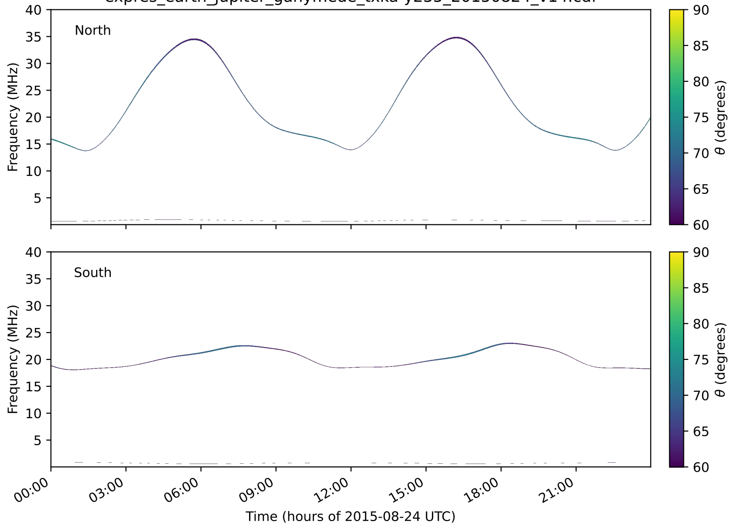
expres_earth_jupiter_ganymede_txka-y235_20150824_v14.cdf
