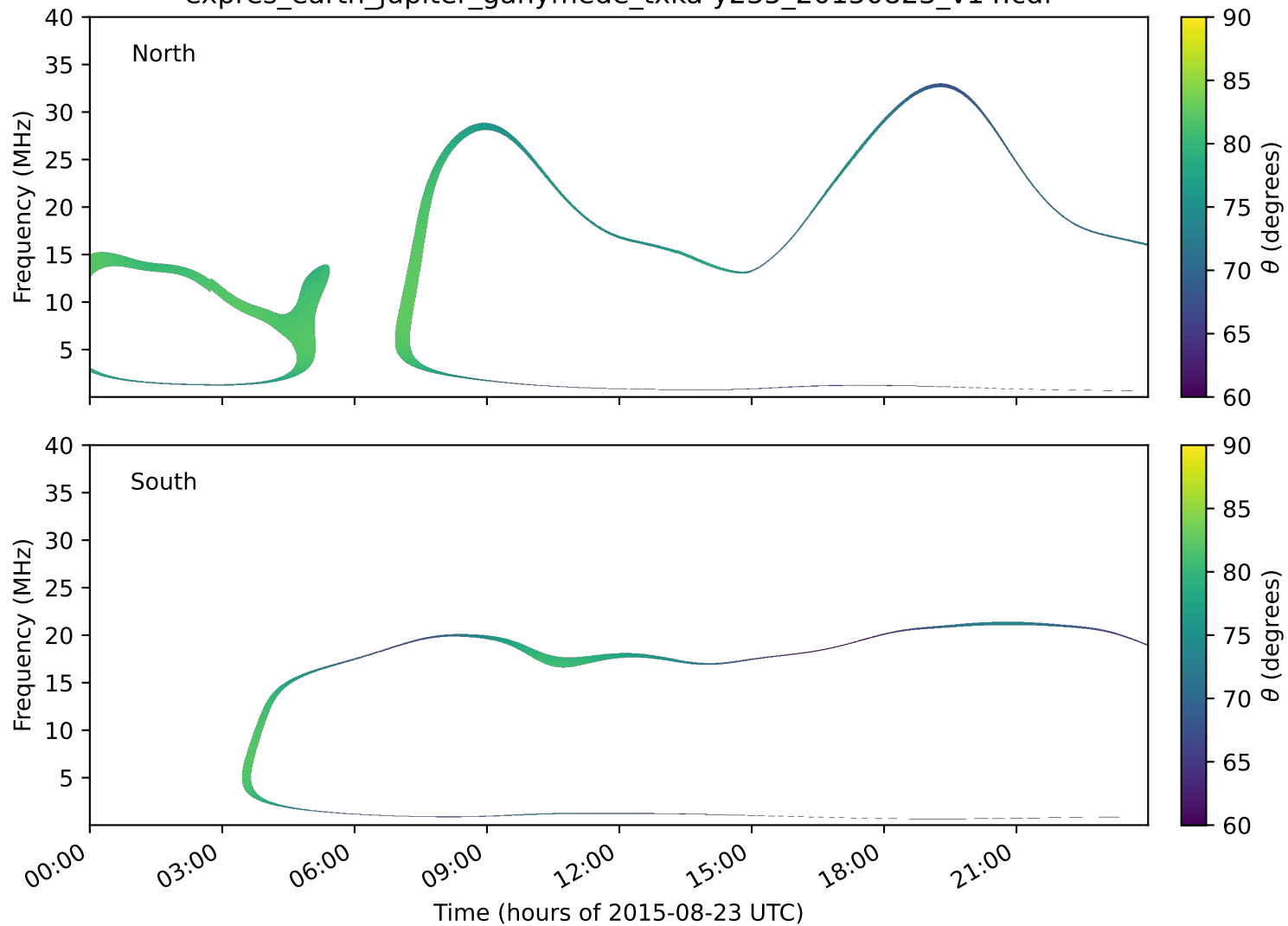
expres_earth_jupiter_ganymede_txka-y235_20150823_v14.cdf
