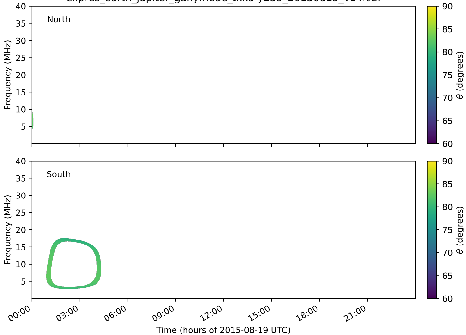
expres_earth_jupiter_ganymede_txka-y235_20150819_v14.cdf
