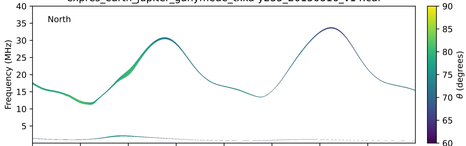
expres_earth_jupiter_ganymede_txka-y235_20150816_v14.cdf
