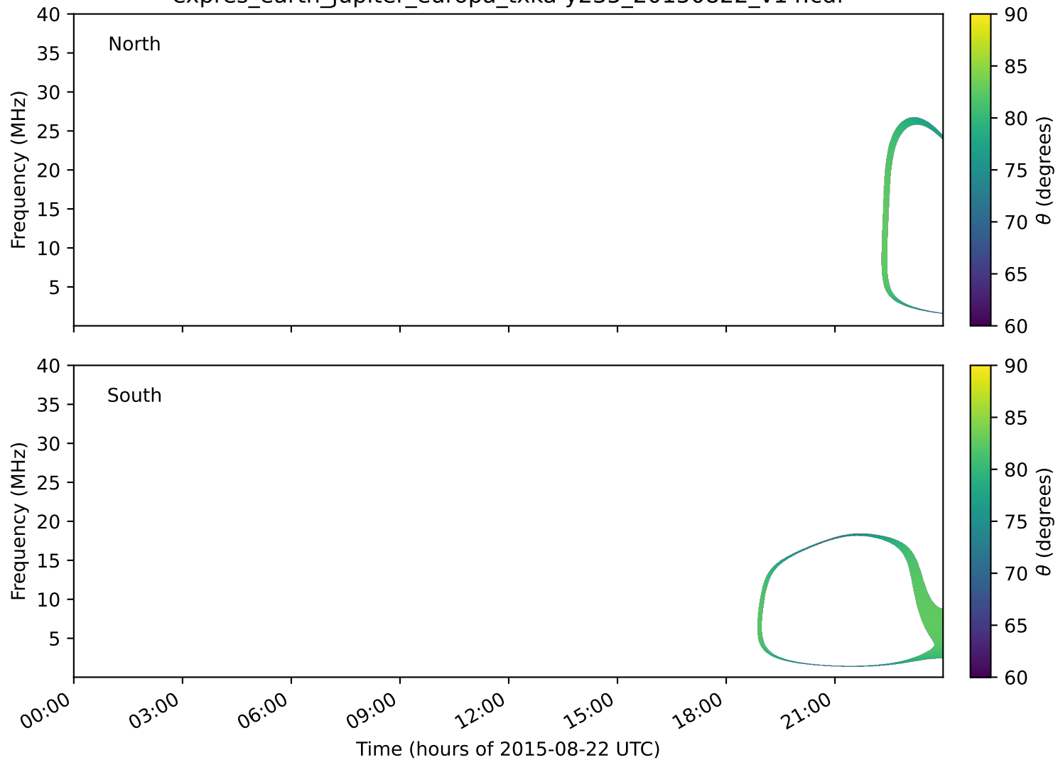
expres_earth_jupiter_europa_txka-y235_20150822_v14.cdf
