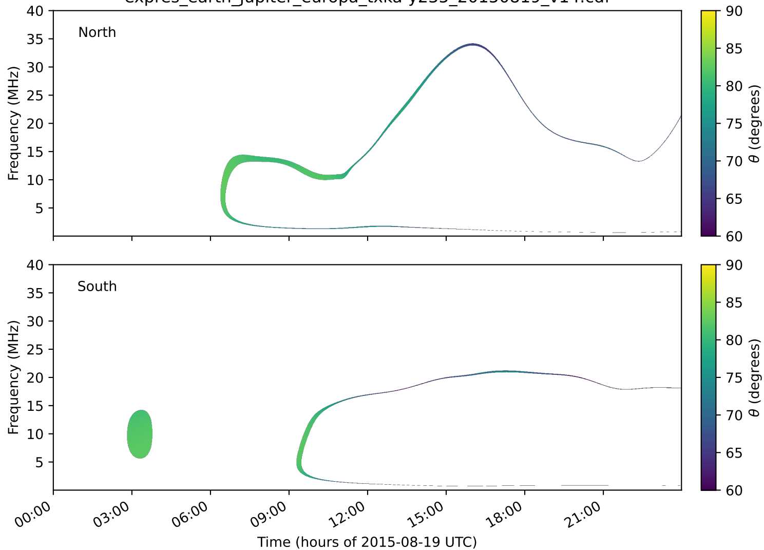
expres_earth_jupiter_europa_txka-y235_20150819_v14.cdf
