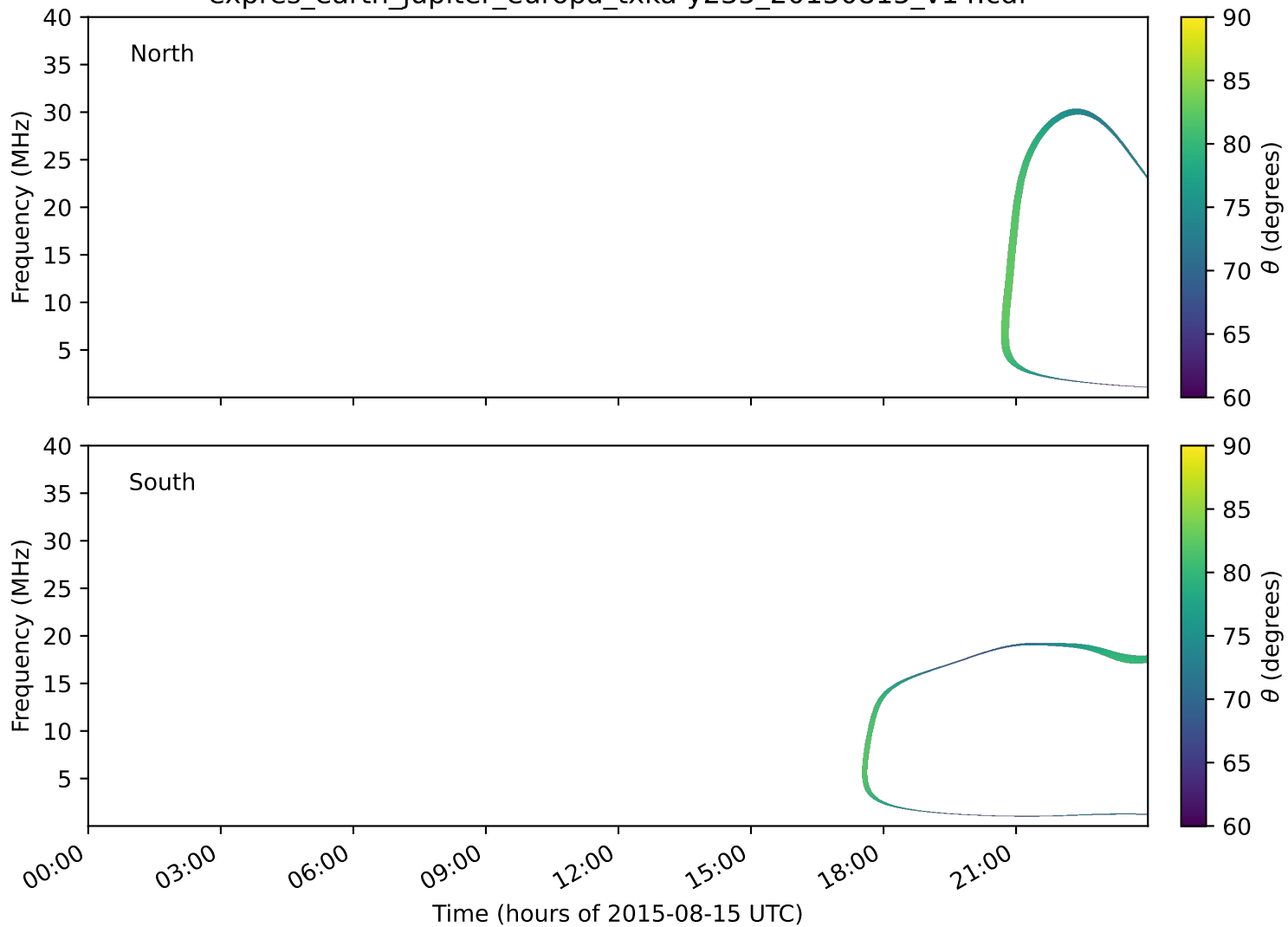
expres_earth_jupiter_europa_txka-y235_20150815_v14.cdf
