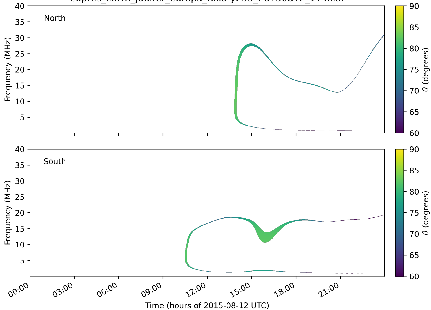
expres_earth_jupiter_europa_txka-y235_20150812_v14.cdf
