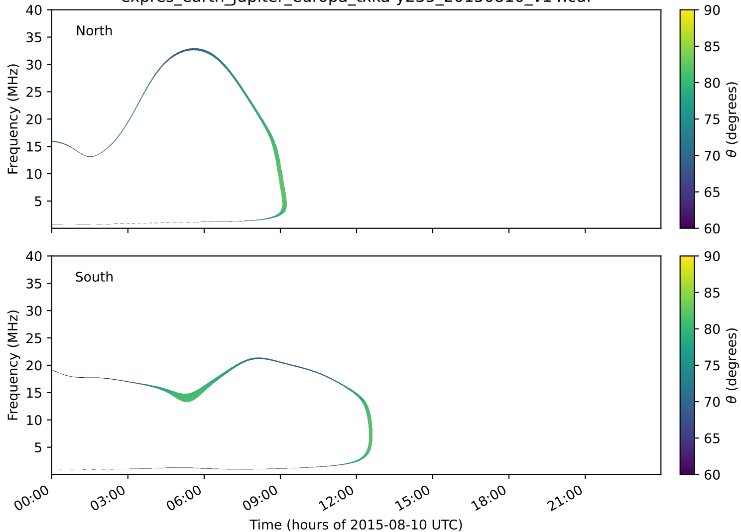
expres_earth_jupiter_europa_txka-y235_20150810_v14.cdf
