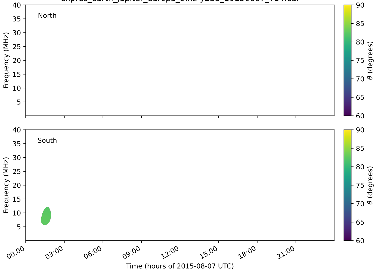
expres_earth_jupiter_europa_txka-y235_20150807_v14.cdf
