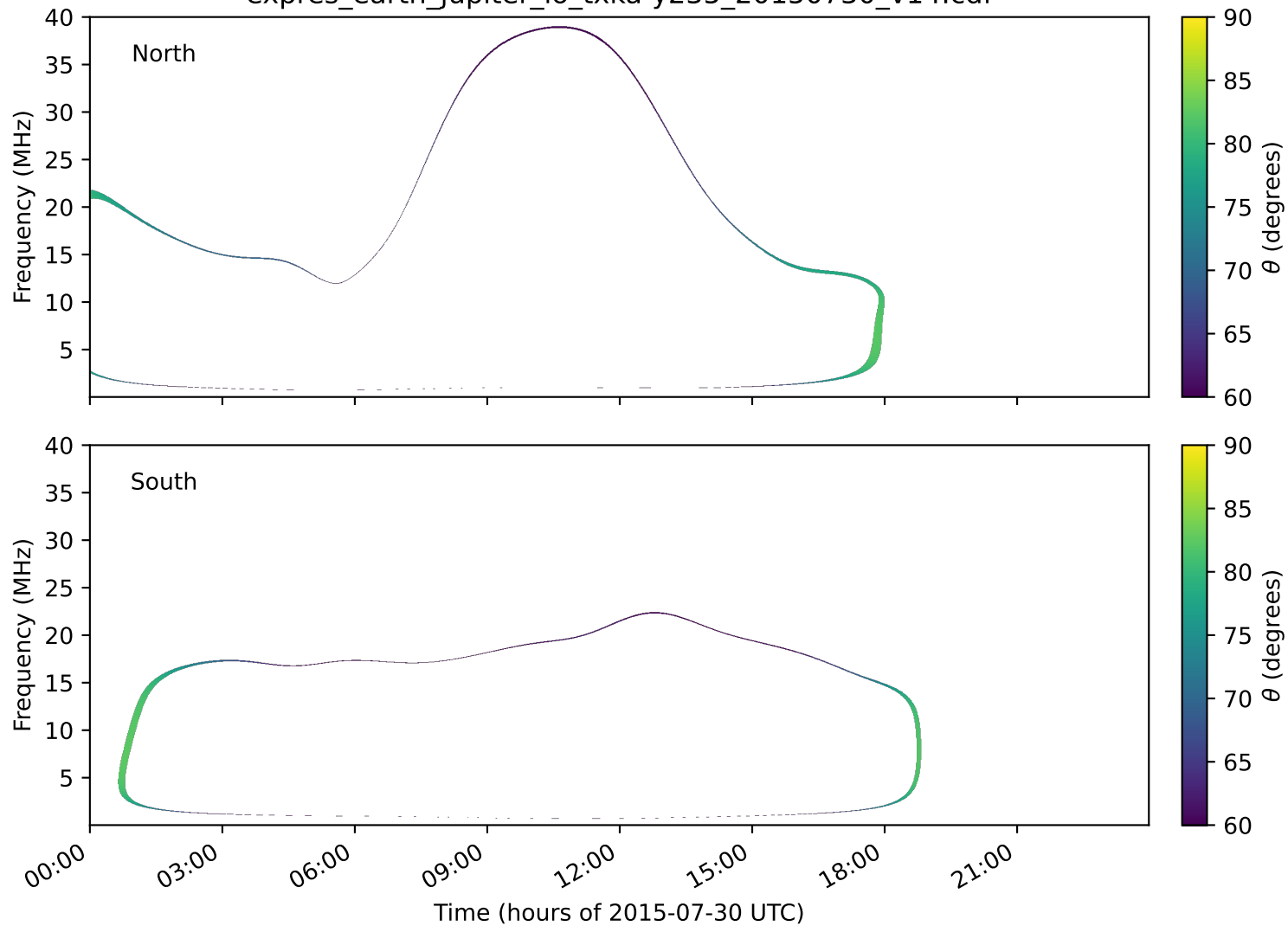
expres_earth_jupiter_io_txka-y235_20150730_v14.cdf
