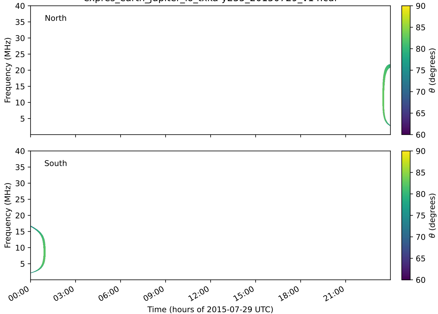
expres_earth_jupiter_io_txka-y235_20150729_v14.cdf
