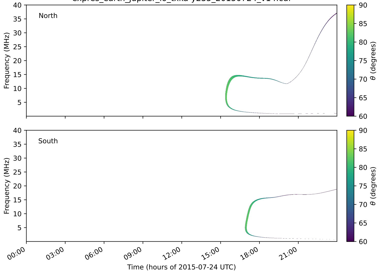
expres_earth_jupiter_io_txka-y235_20150724_v14.cdf
