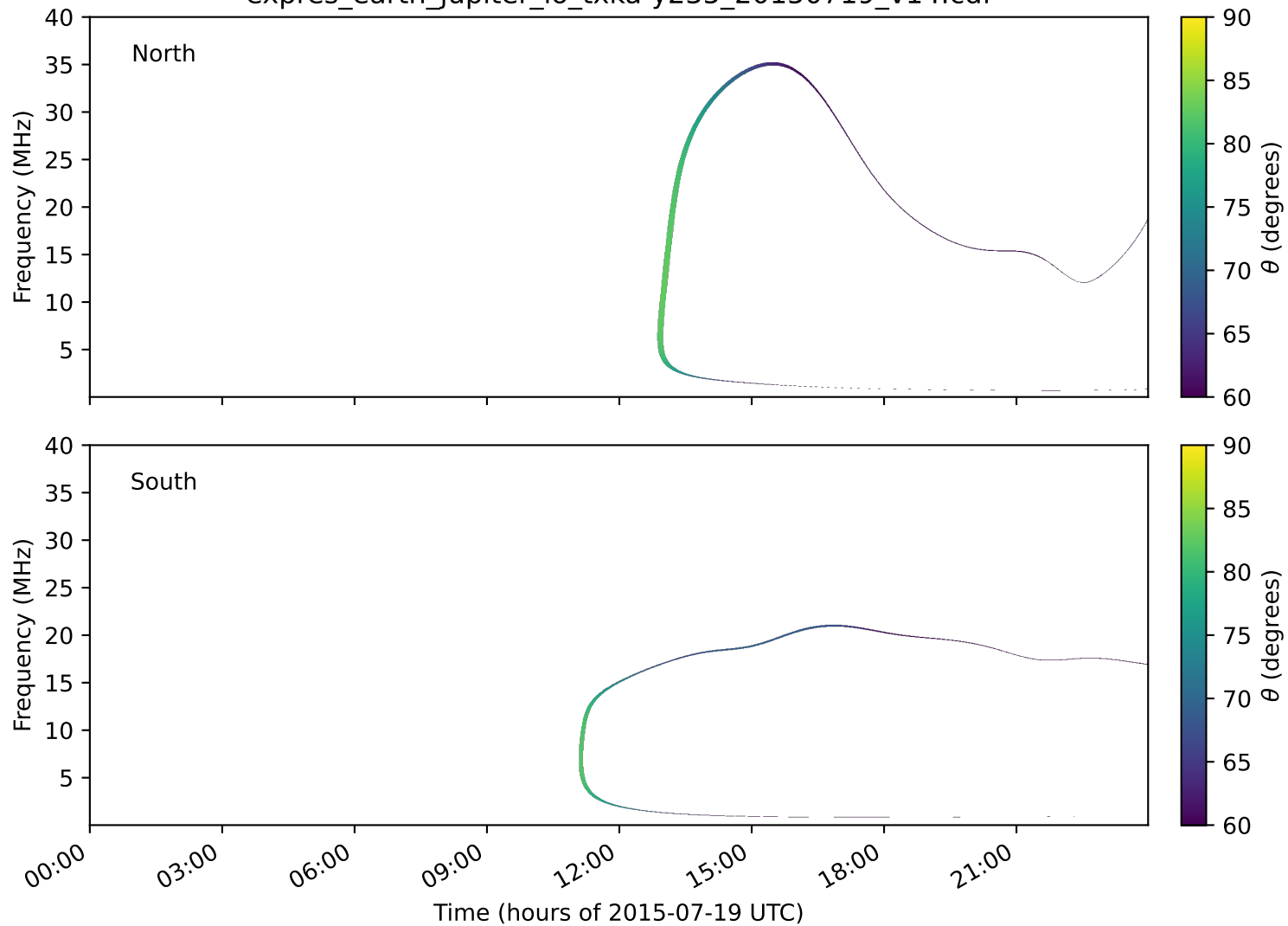
expres_earth_jupiter_io_txka-y235_20150719_v14.cdf
