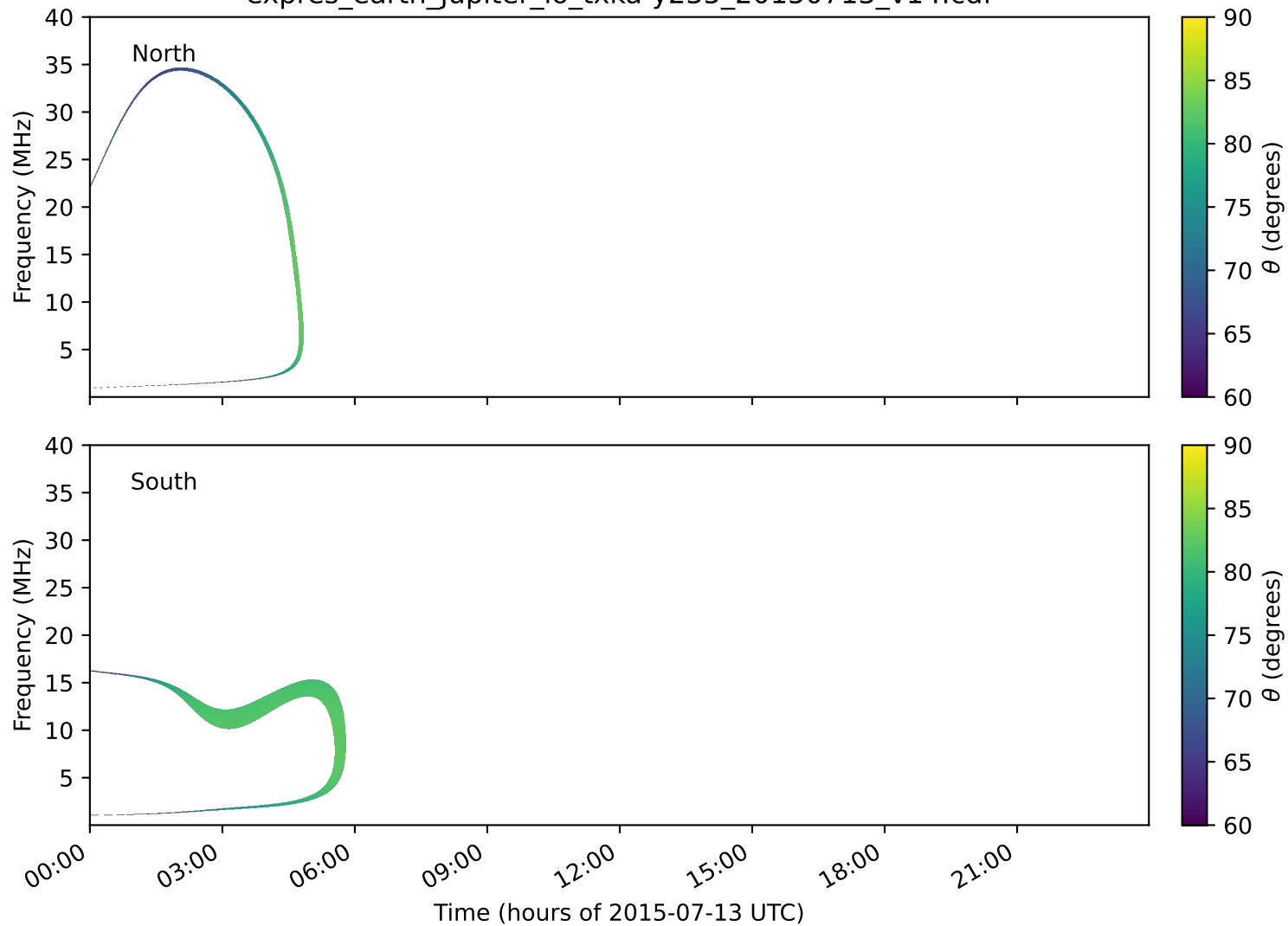
expres_earth_jupiter_io_txka-y235_20150713_v14.cdf
