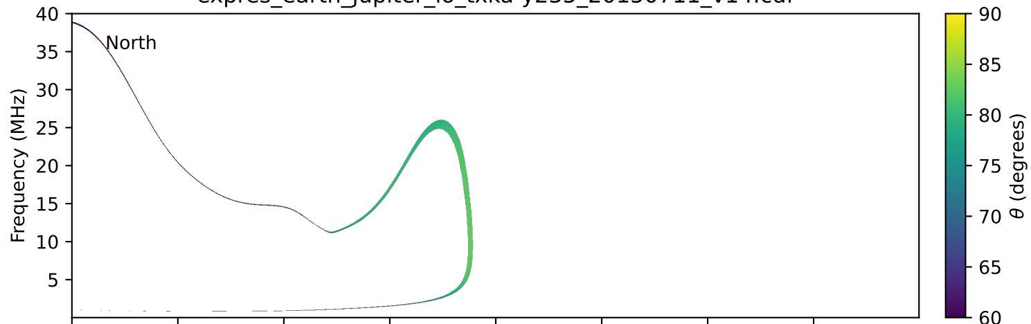
expres_earth_jupiter_io_txka-y235_20150711_v14.cdf
