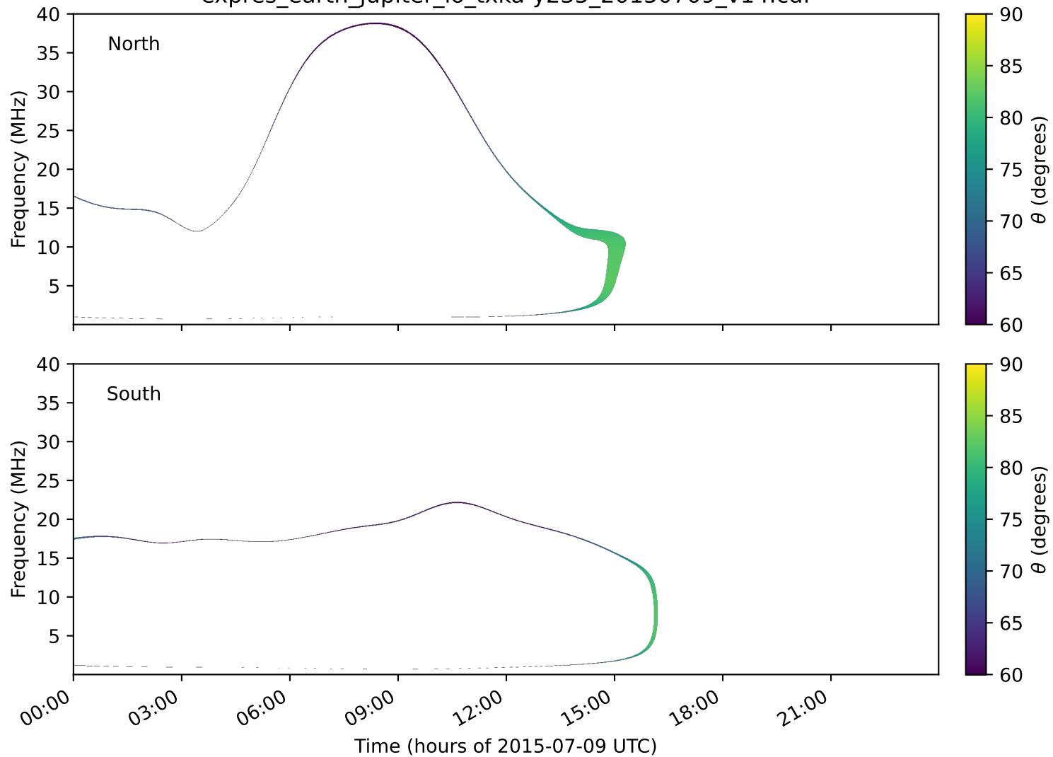
expres_earth_jupiter_io_txka-y235_20150709_v14.cdf
