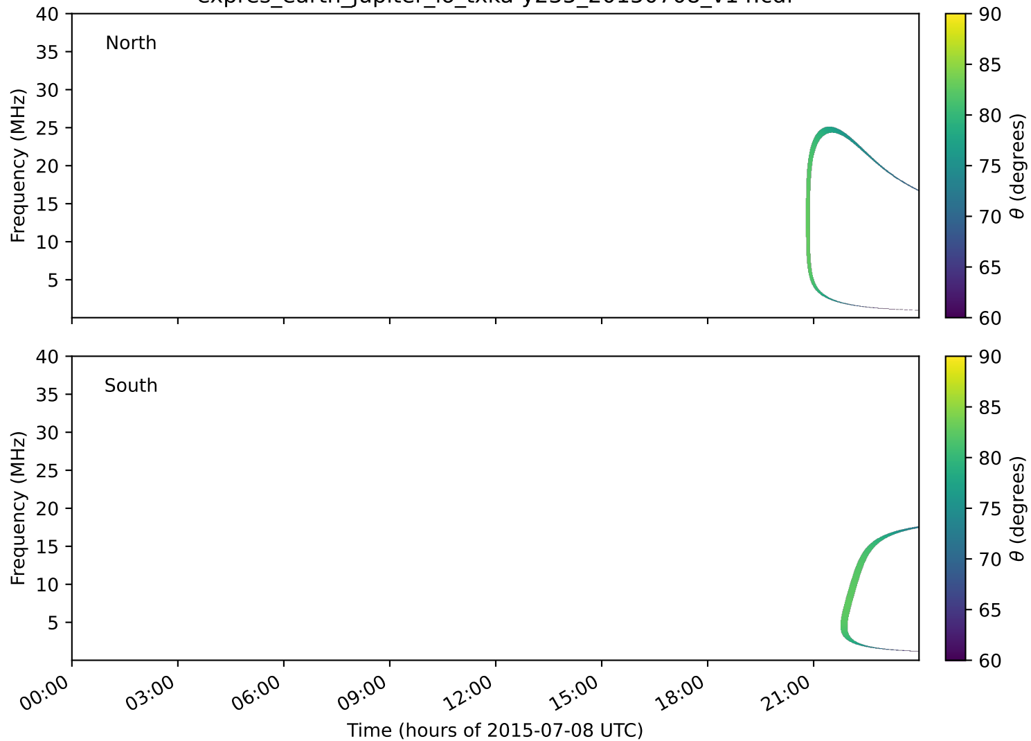
expres_earth_jupiter_io_txka-y235_20150708_v14.cdf
