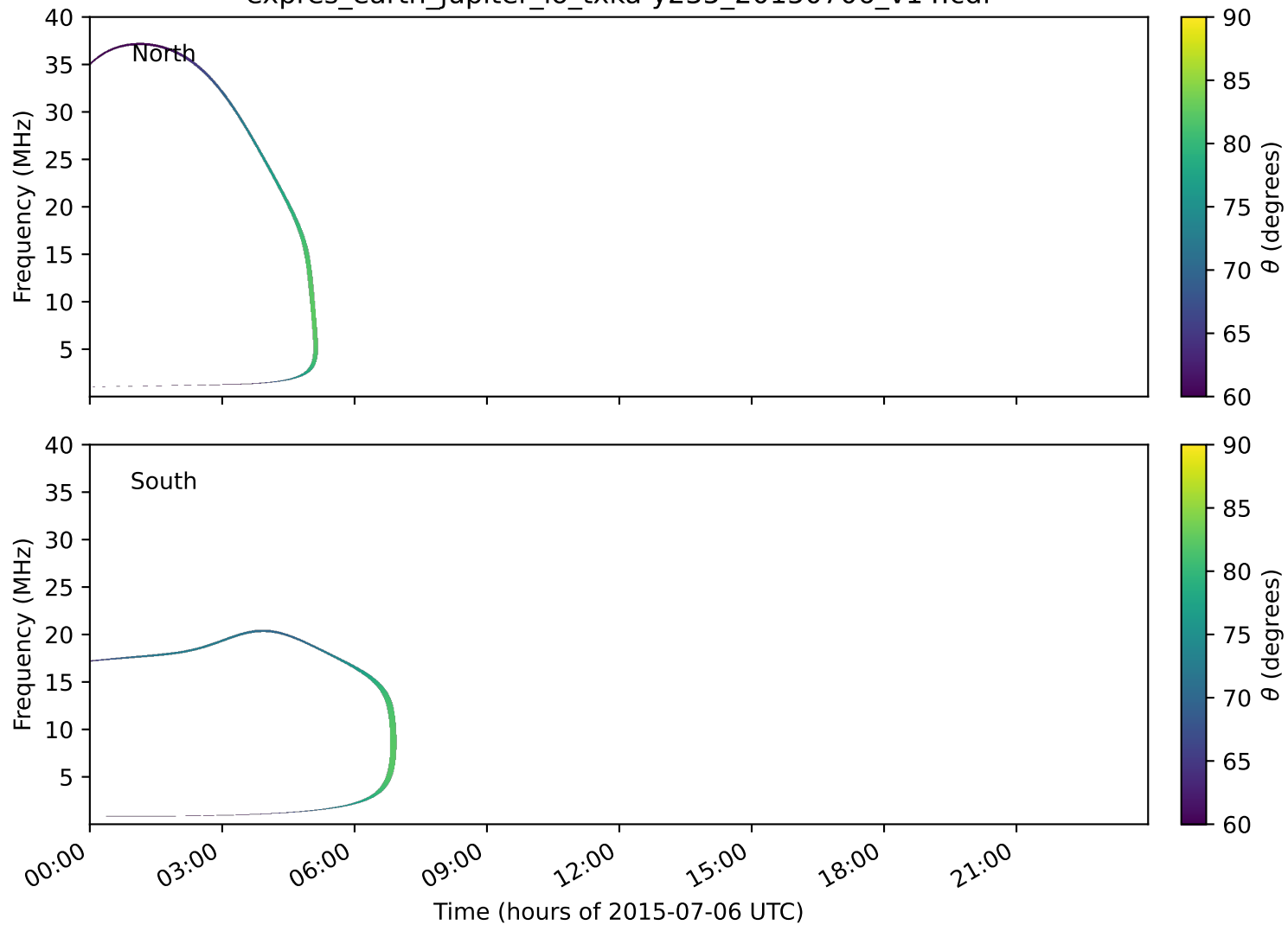
expres_earth_jupiter_io_txka-y235_20150706_v14.cdf
