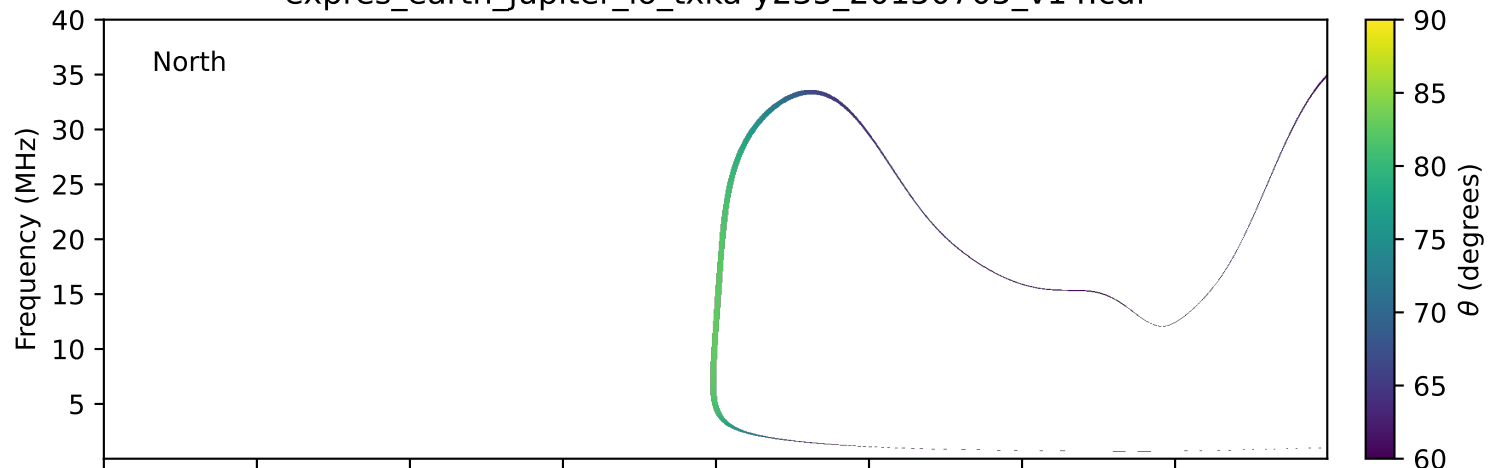
expres_earth_jupiter_io_txka-y235_20150705_v14.cdf
