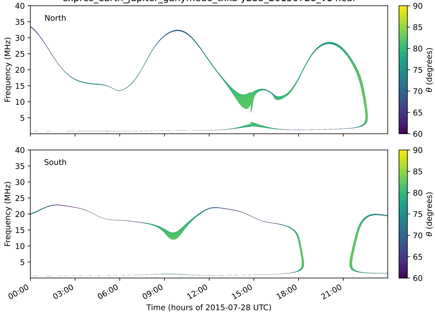
expres_earth_jupiter_ganymede_txka-y235_20150728_v14.cdf
