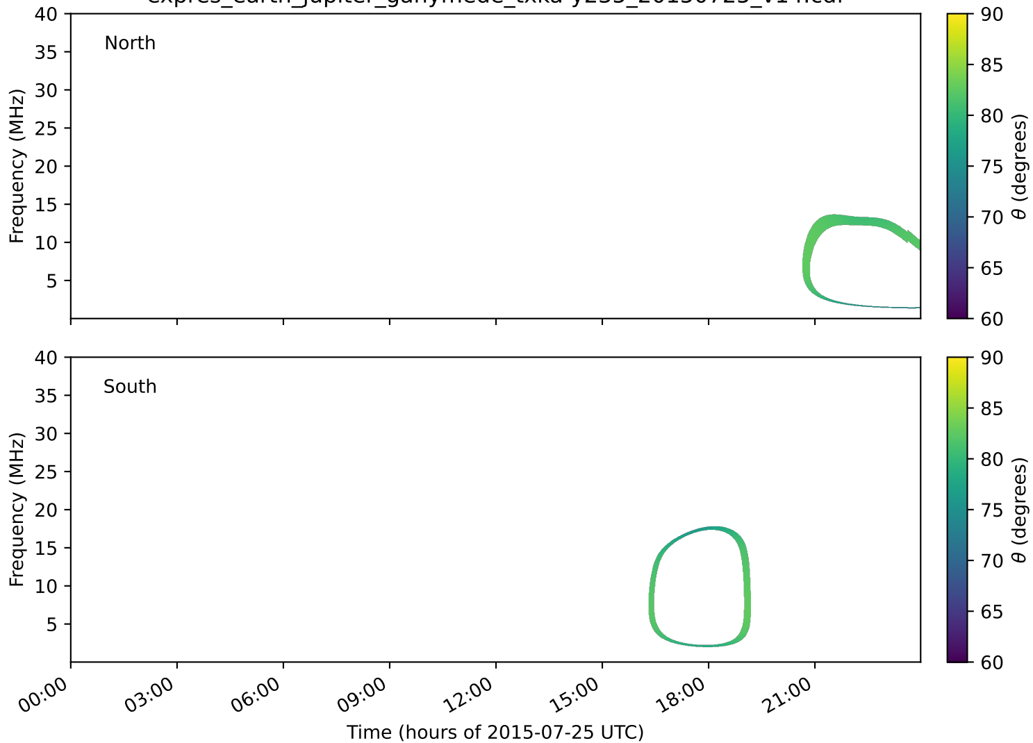
expres_earth_jupiter_ganymede_txka-y235_20150725_v14.cdf
