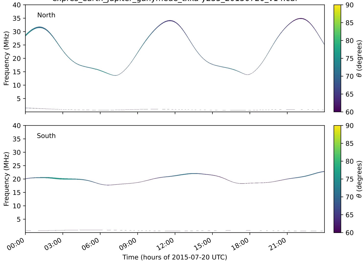
expres_earth_jupiter_ganymede_txka-y235_20150720_v14.cdf
