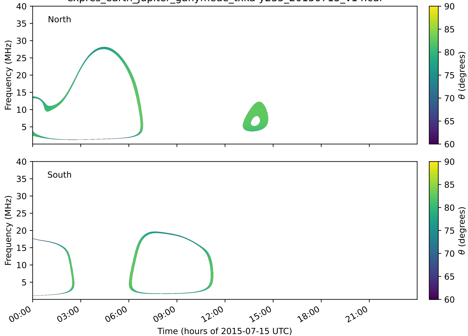
expres_earth_jupiter_ganymede_txka-y235_20150715_v14.cdf
