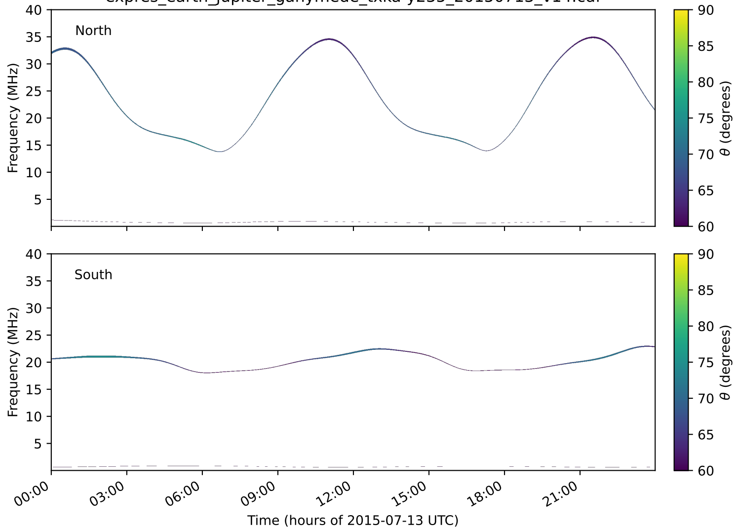
expres_earth_jupiter_ganymede_txka-y235_20150713_v14.cdf
