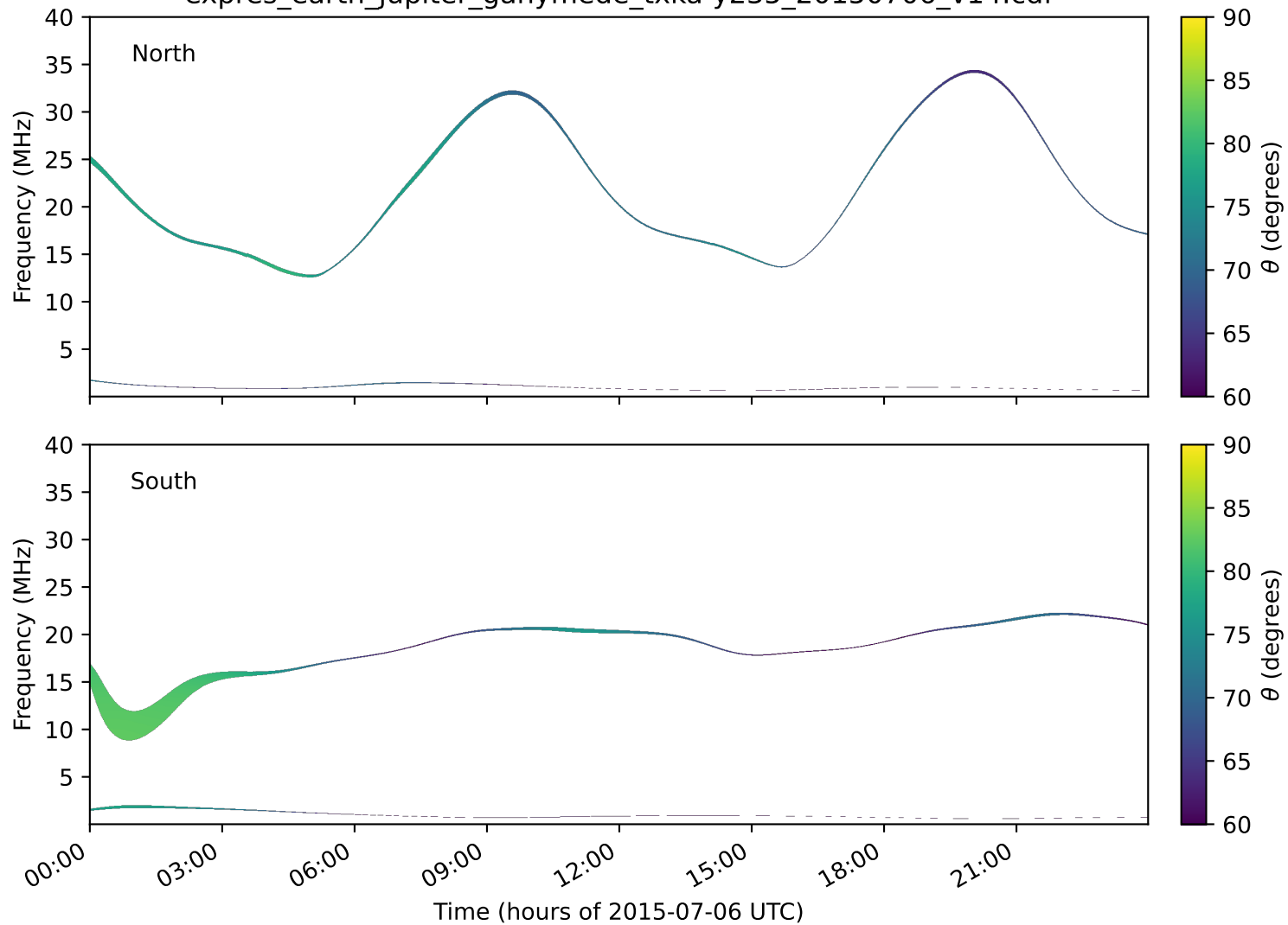
expres_earth_jupiter_ganymede_txka-y235_20150706_v14.cdf
