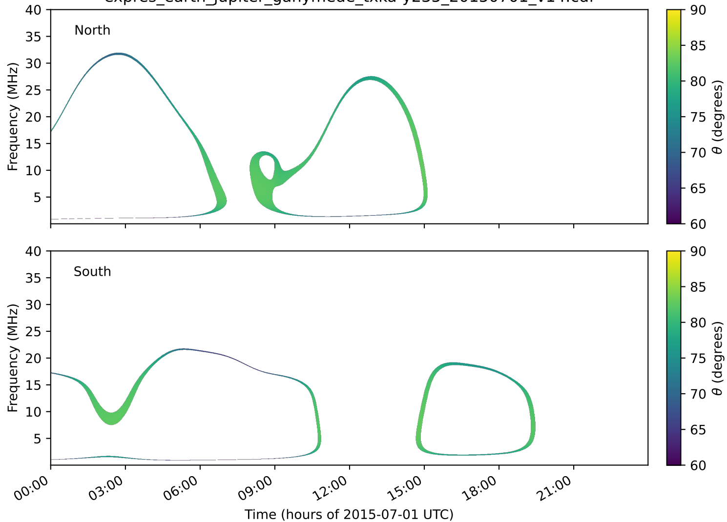
expres_earth_jupiter_ganymede_txka-y235_20150701_v14.cdf
