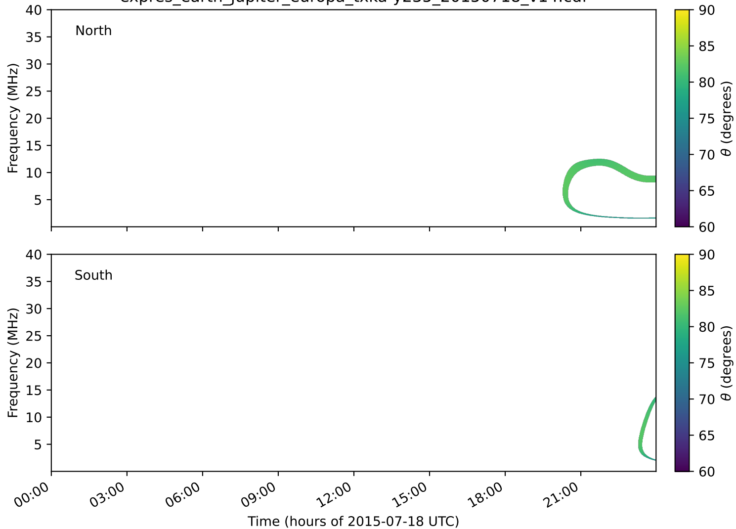
expres_earth_jupiter_europa_txka-y235_20150718_v14.cdf
