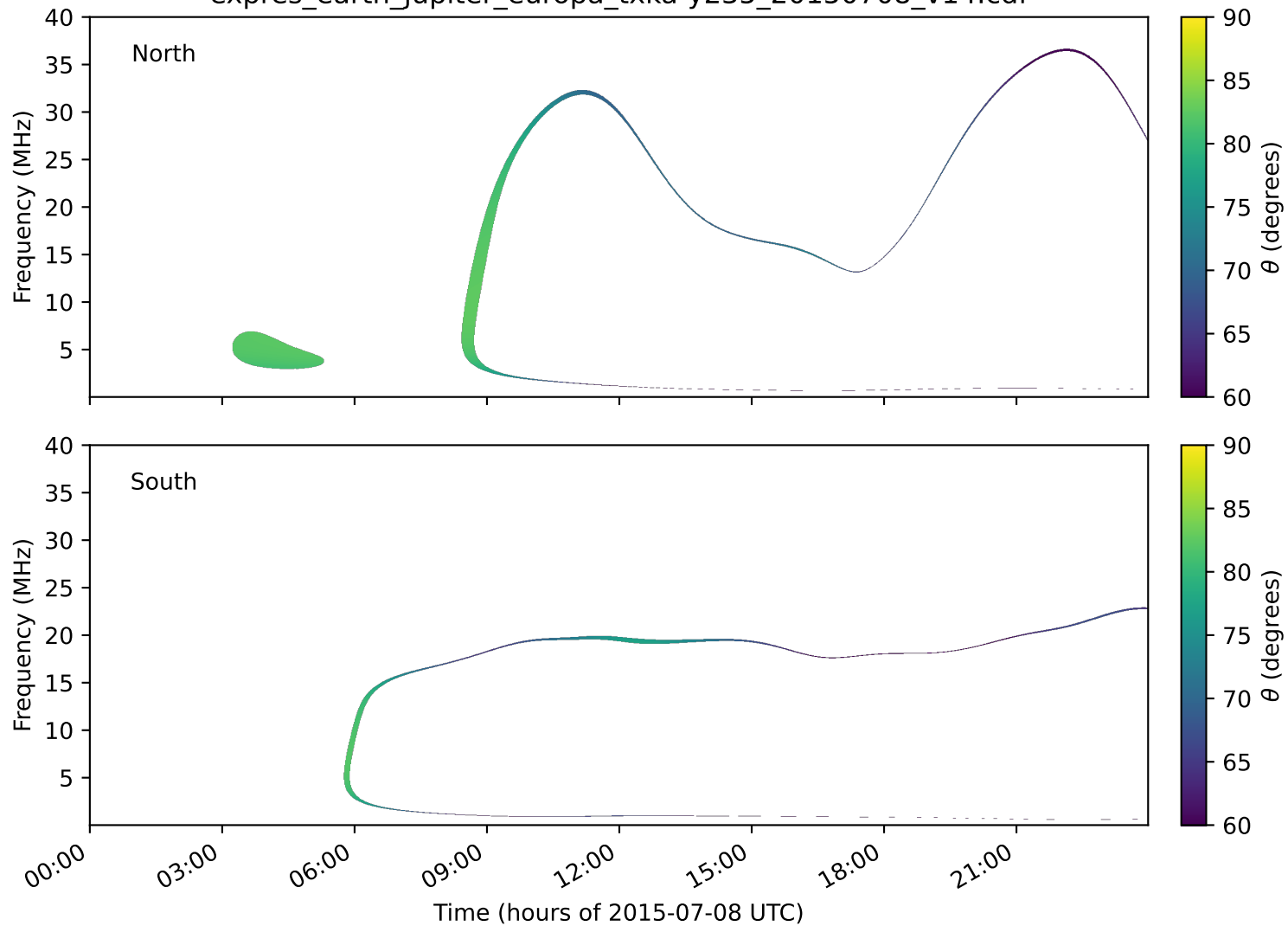
expres_earth_jupiter_europa_txka-y235_20150708_v14.cdf
