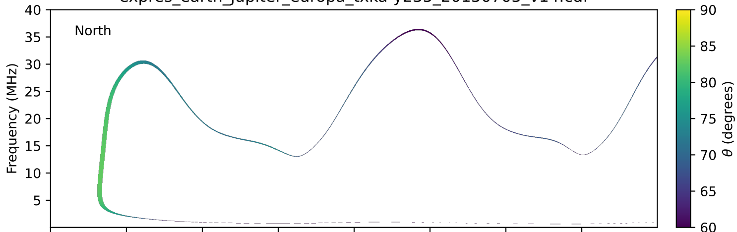
expres_earth_jupiter_europa_txka-y235_20150705_v14.cdf
