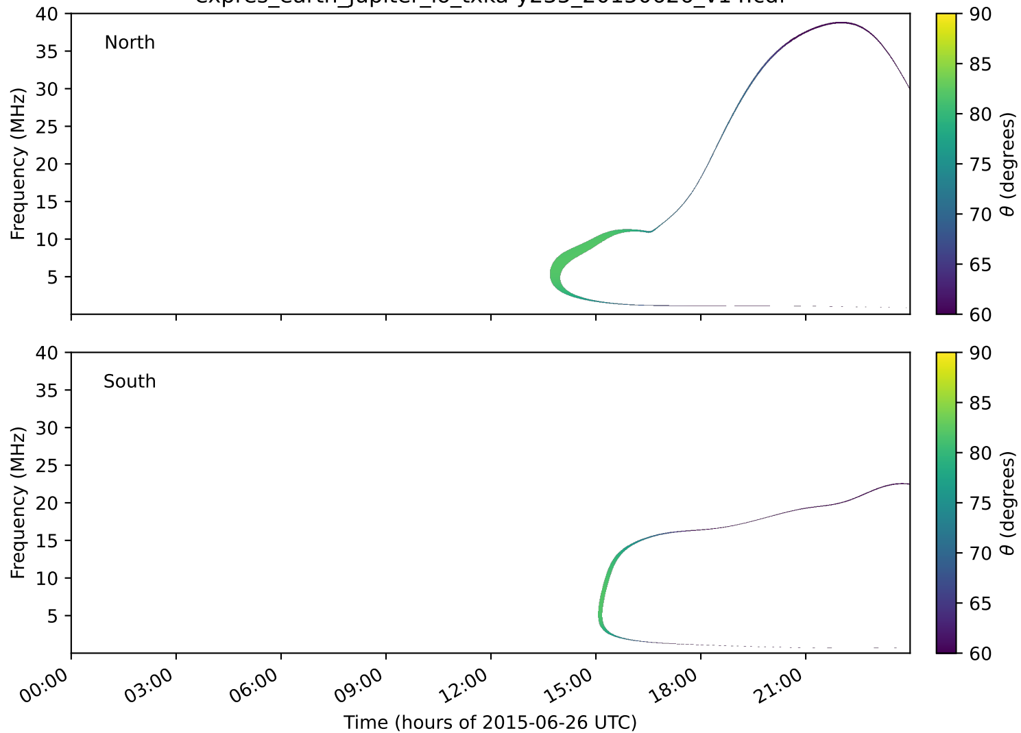
expres_earth_jupiter_io_txka-y235_20150626_v14.cdf
