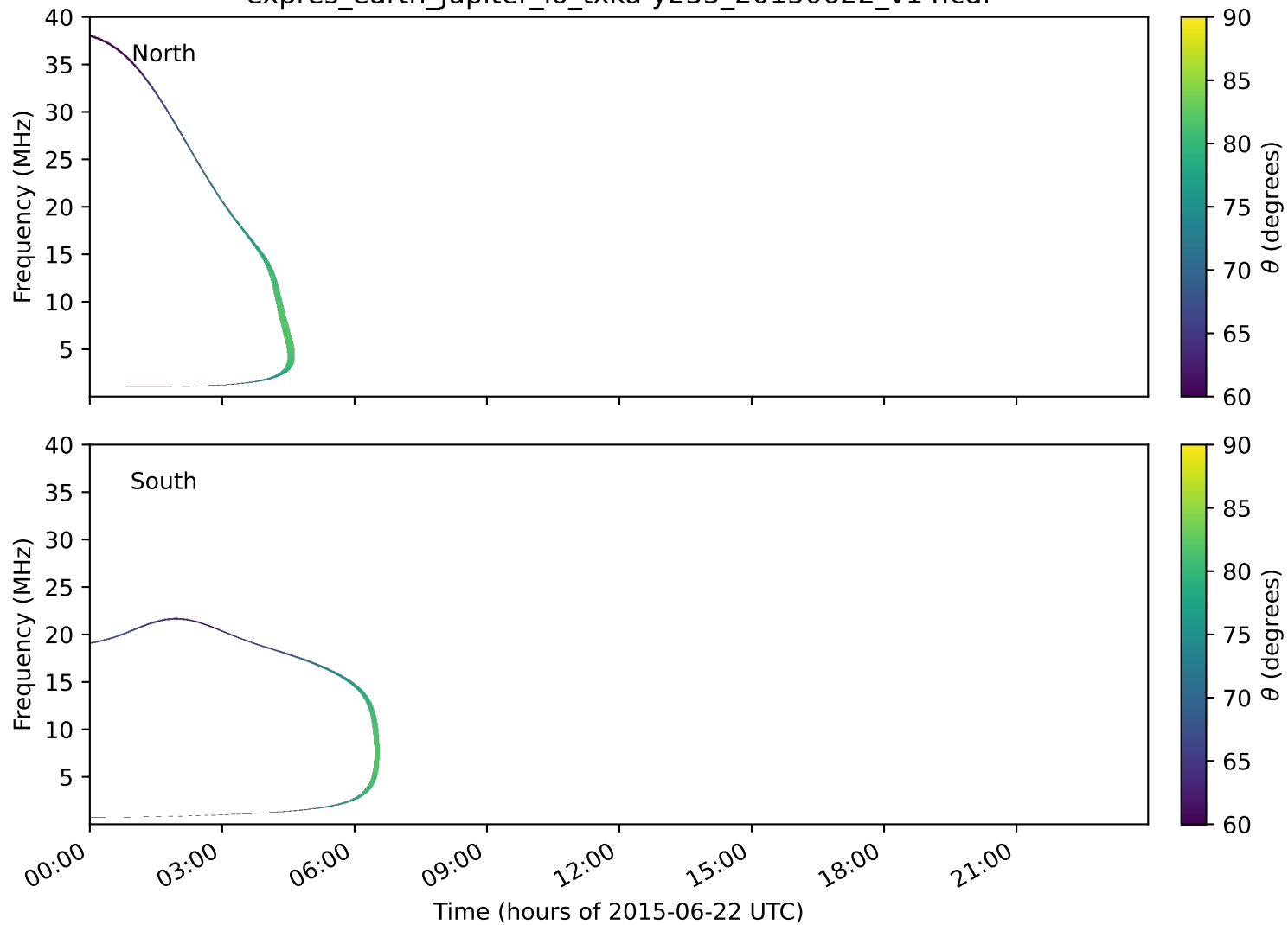
expres_earth_jupiter_io_txka-y235_20150622_v14.cdf
